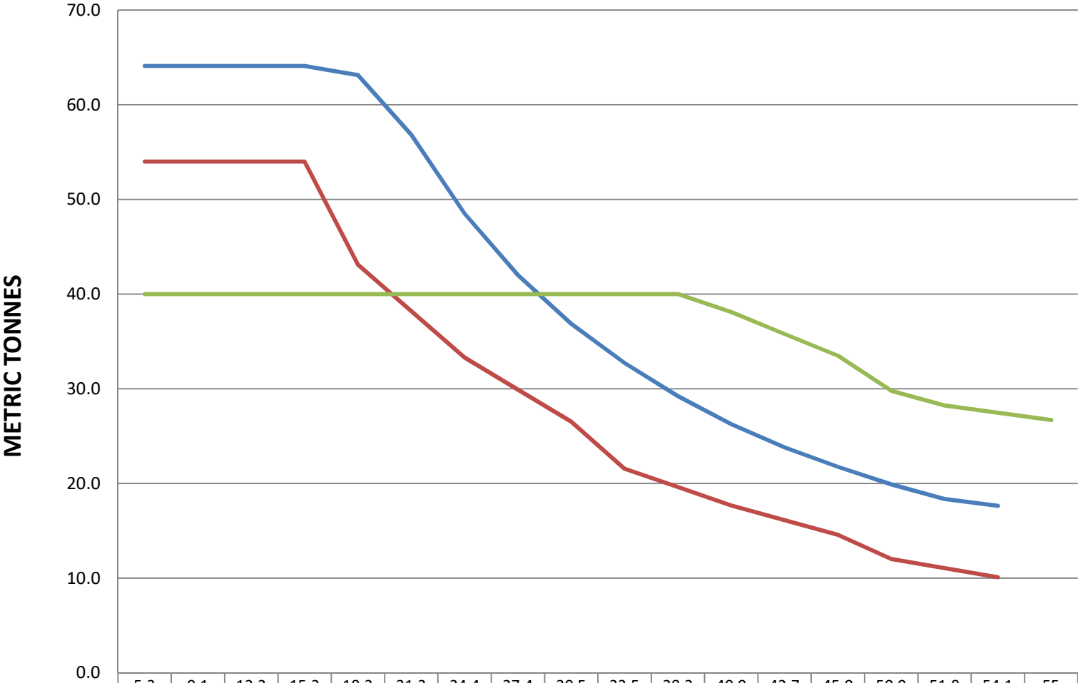
55.0 m (180 Ft) Boom 96.5 Tonne Counterweight | Two Fall
